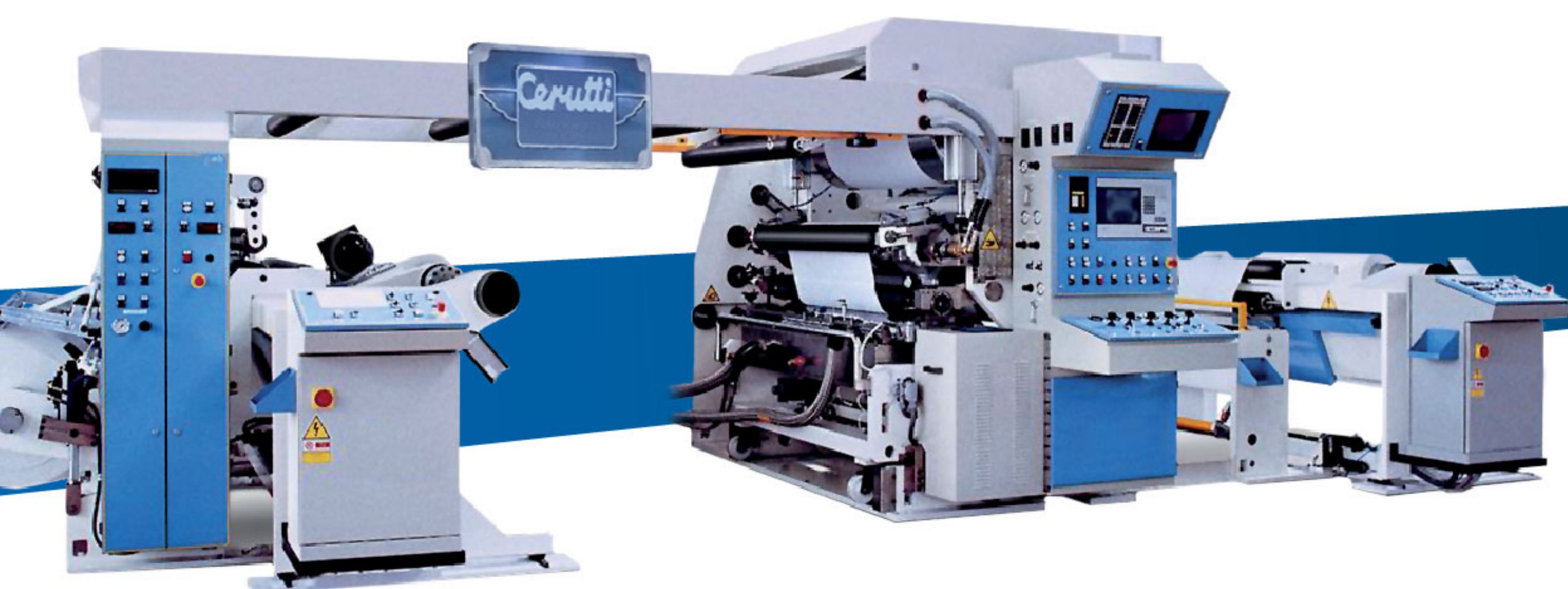
Solventless coating and laminating unit
