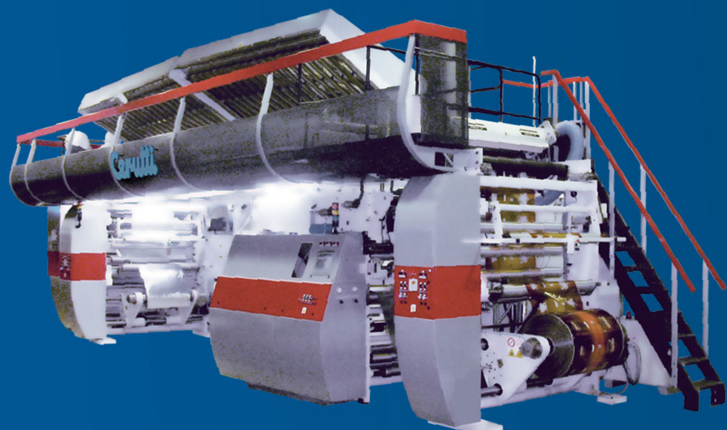
Dry laminating machine
